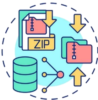
Data Compression
